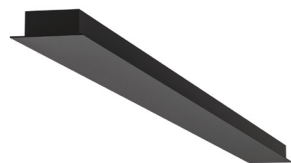
built-up
